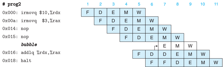
Figure 4.47 Pipelined execution of prog2 using stalls. After decoding the addq instruction in cycle 6, the stall control detects a data hazard due to the pending write to register %rax in the write-back stage. It injects a bubble into the execute stage and repeats the decoding of the addq instruction in cycle 7. In effect, the machine has dynamically inserted a nop instruction, giving a flow similar to that shown for prog1 (Figure 4.43).
