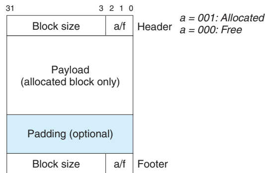
Format of heap block that uses a boundary tag.
